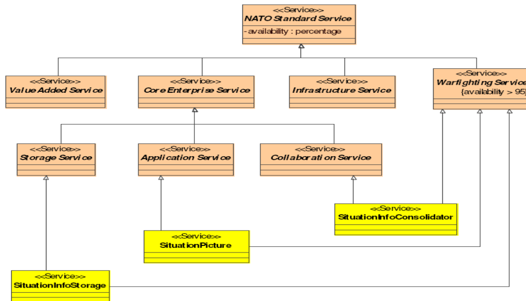
Figure 4-17, Example of a service taxonomy
