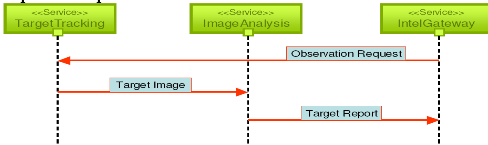
Figure 4-21, Example of a Service Behaviour sequence diagram
